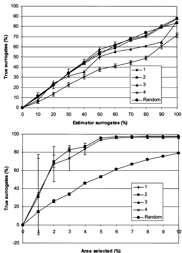
Figure 3. Surrogacy graphs for Queensland: (top) Queensland at the 0.01^\circ \times 0.01^\circ longitude \times latitude scale; (bottom) Queensland at the 0.10^\circ \times 0.10^\circ longitude \times latitude scale. For further detail, see the legend for Fig. 1.
