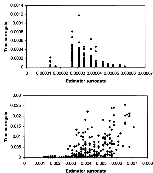
Figure 5. Marginal species representation plots: (top) Québec, environmental surrogate set 1 at the 0.01^\circ \times 0.01^\circ longitude \times latitude scale (each point represents the marginal representation of the estimator surrogates [x-axis] and true surrogates [y-axis] of an individual cell) and (bottom) Queensland, environmental surrogate set 1 at the 0.10^\circ \times 0.10^\circ longitude \times latitude scale.
