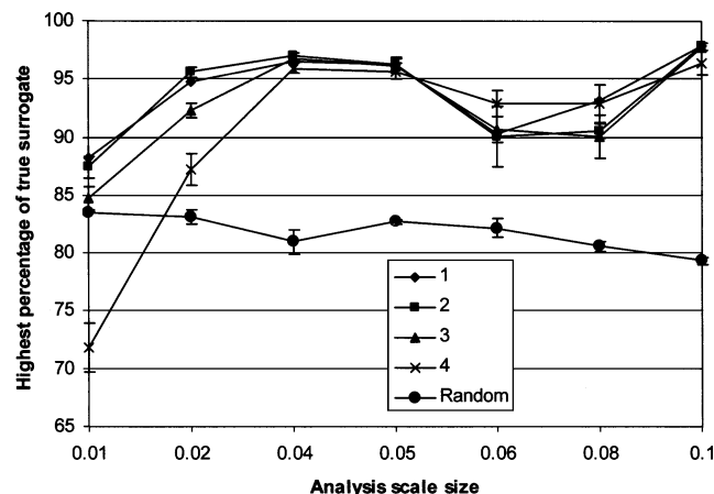
Figure 4. Queensland scale analysis: x-axis, cell boundary size in longitude/latitude, and y-axis, representation level of true surrogates when 100% representation of estimator surrogates has been achieved. The error bars show standard deviations from 100 different runs rather than standard errors because the latter were too small to be depicted.
